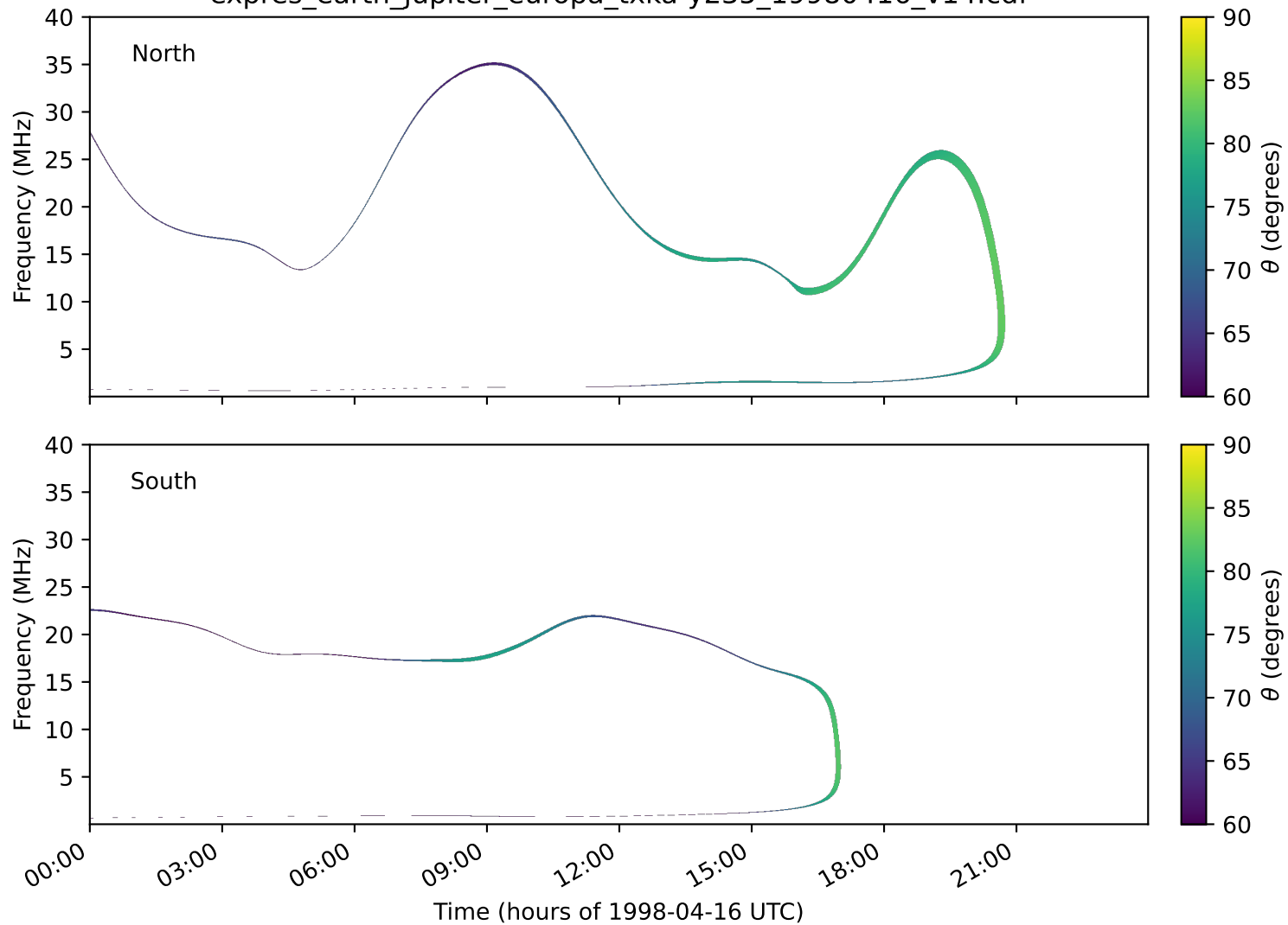
expres_earth_jupiter_europa_txka-y235_19980416_v14.cdf
