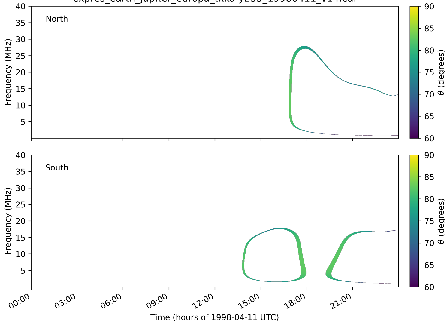
expres_earth_jupiter_europa_txka-y235_19980411_v14.cdf
