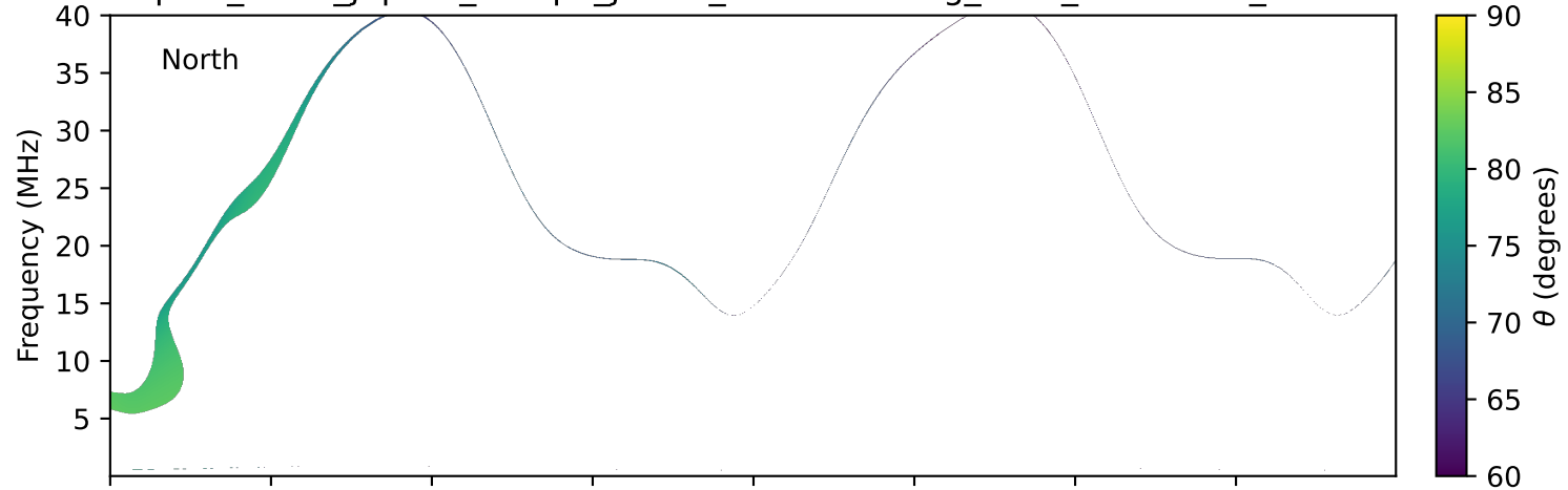
expres_earth_jupiter_europa_jrm33_lossc-wid1deg_3kev_19980426_v11.cdf
