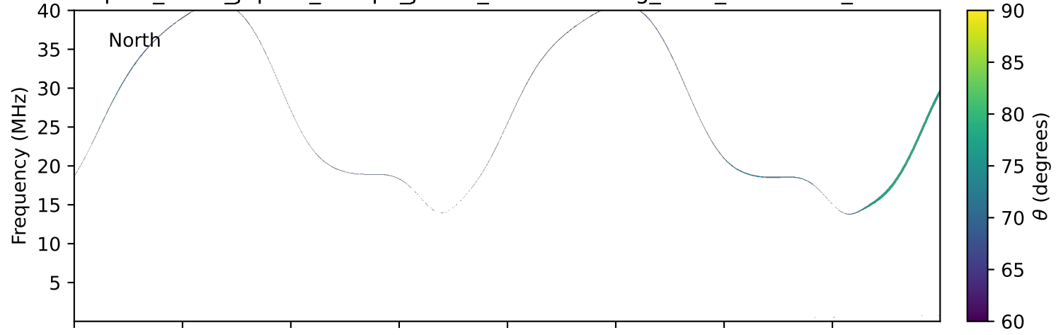
expres_earth_jupiter_europa_jrm33_lossc-wid1deg_3kev_19980405_v11.cdf
