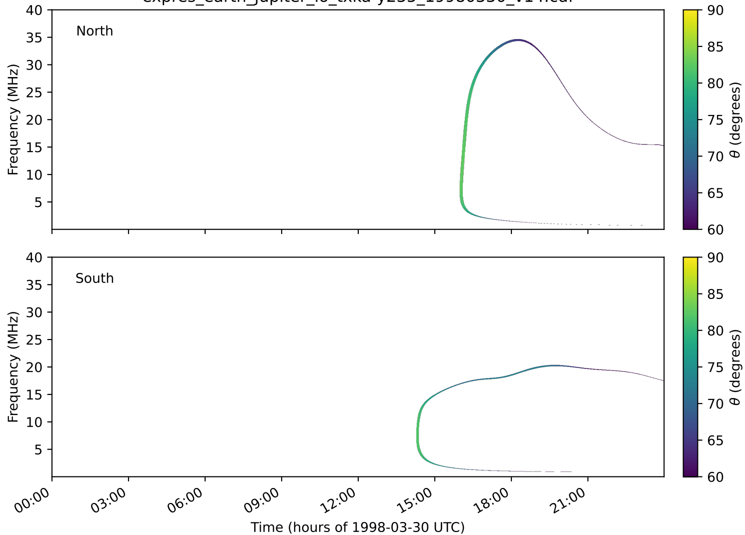
expres_earth_jupiter_io_txka-y235_19980330_v14.cdf
