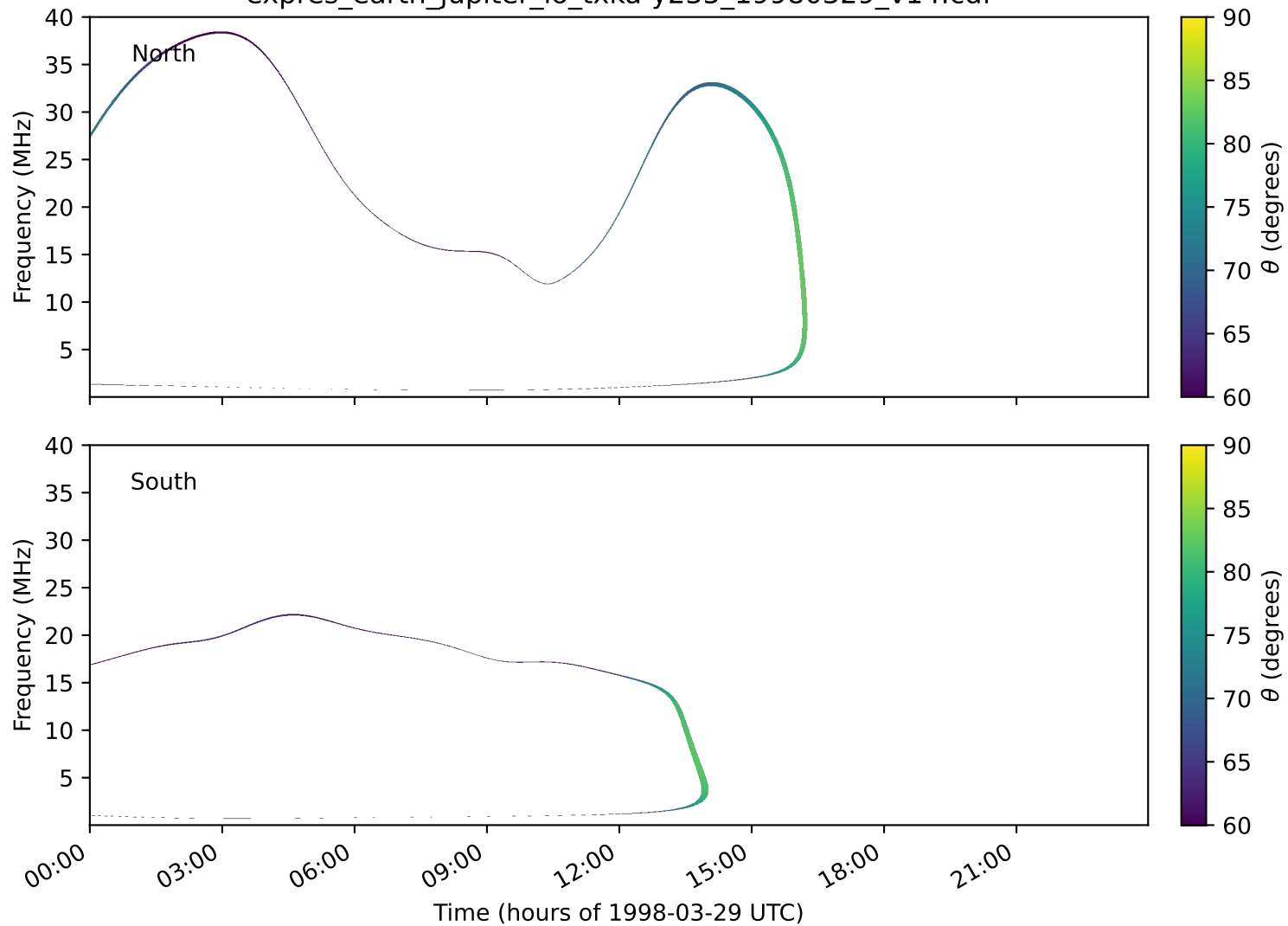
expres_earth_jupiter_io_txka-y235_19980329_v14.cdf
