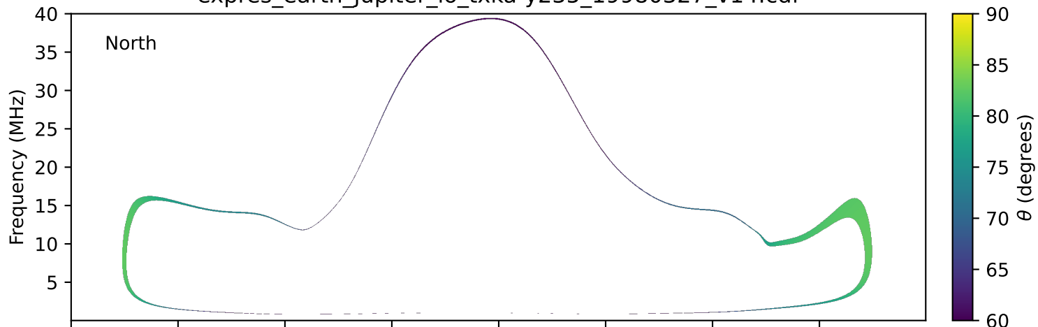
expres_earth_jupiter_io_txka-y235_19980327_v14.cdf
