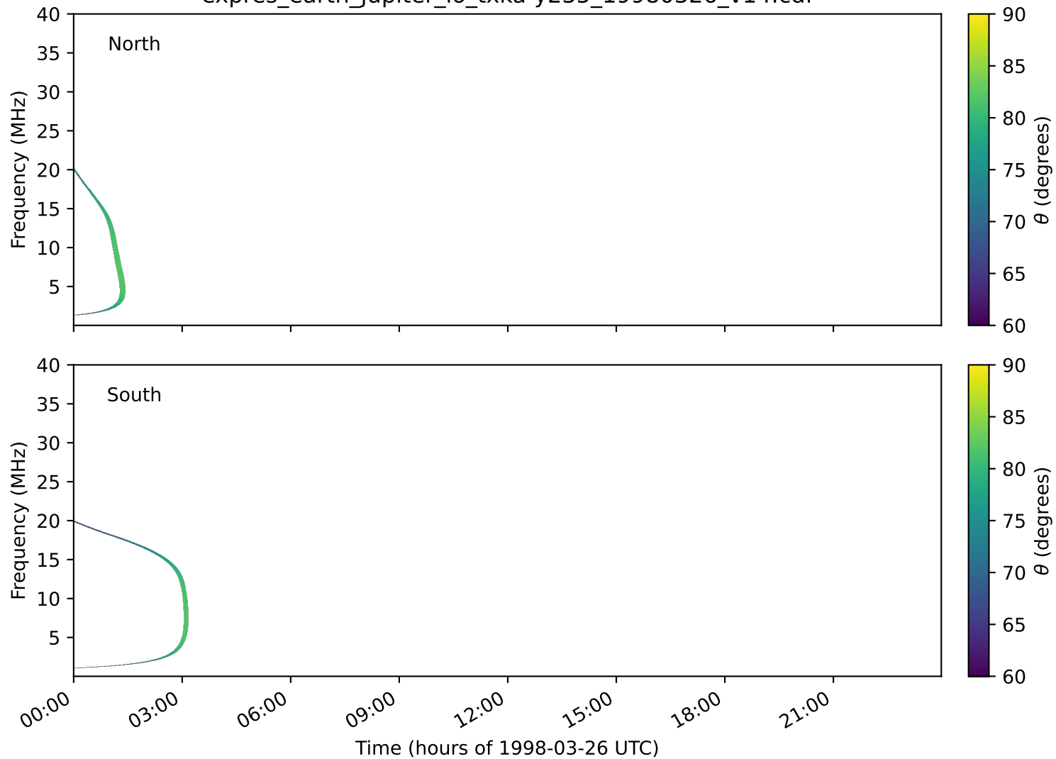
expres_earth_jupiter_io_txka-y235_19980326_v14.cdf
