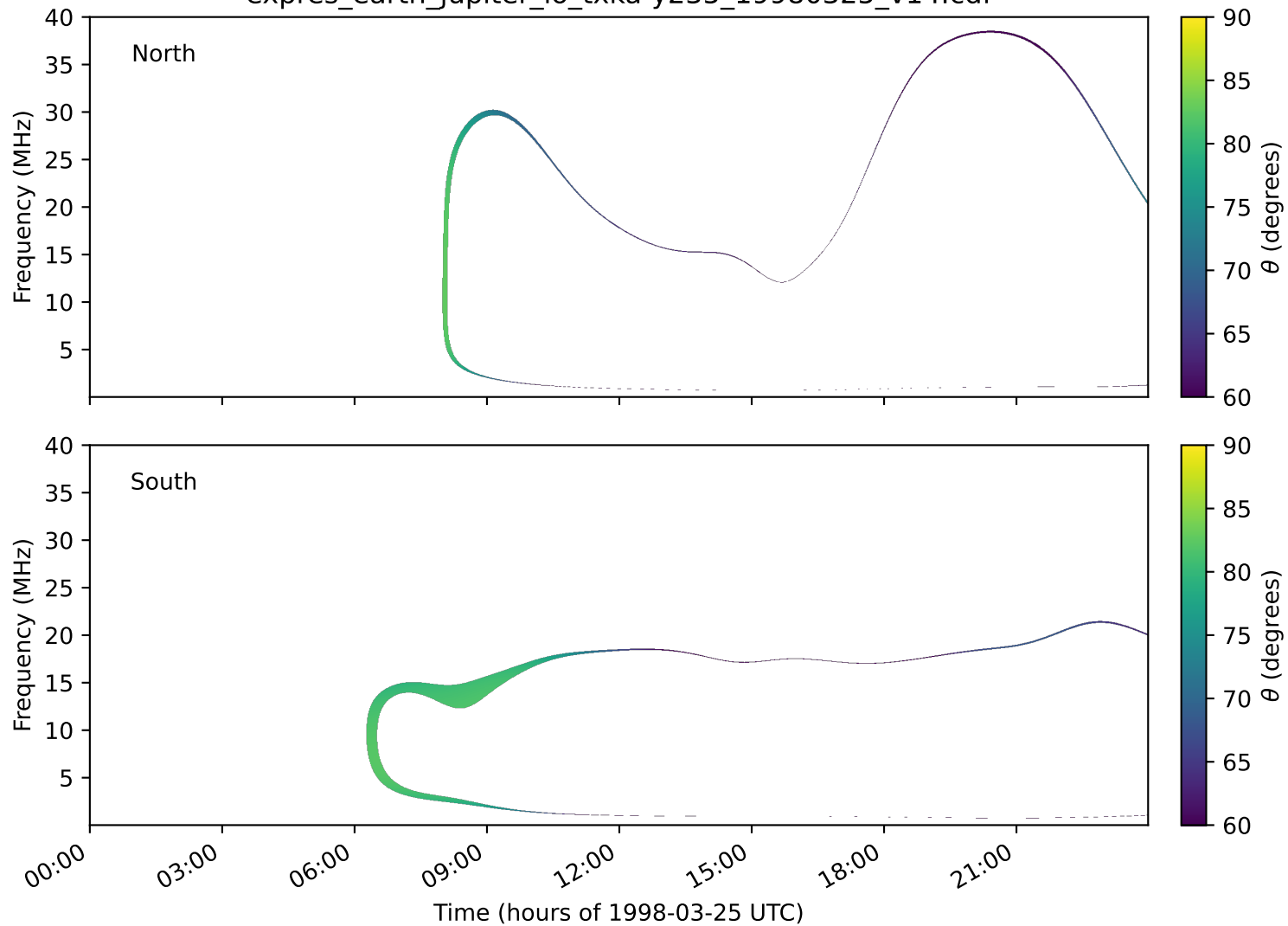
expres_earth_jupiter_io_txka-y235_19980325_v14.cdf
