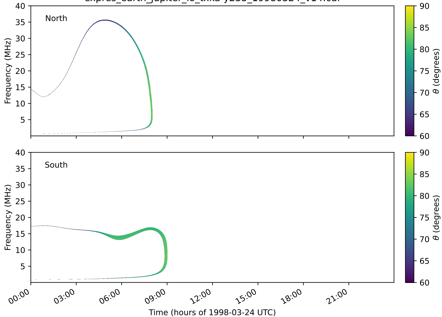
expres_earth_jupiter_io_txka-y235_19980324_v14.cdf
