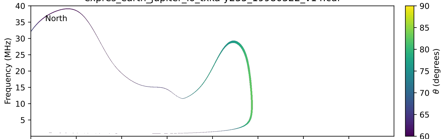
expres_earth_jupiter_io_txka-y235_19980322_v14.cdf
