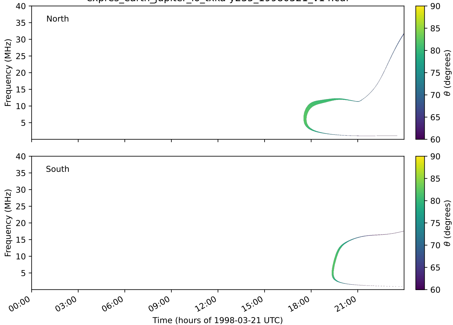
expres_earth_jupiter_io_txka-y235_19980321_v14.cdf
