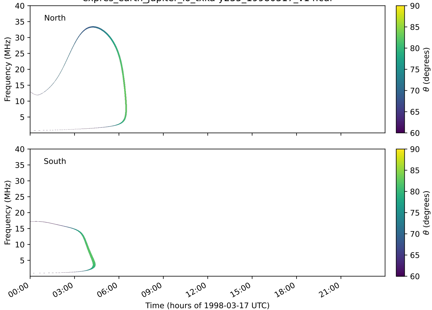
expres_earth_jupiter_io_txka-y235_19980317_v14.cdf
