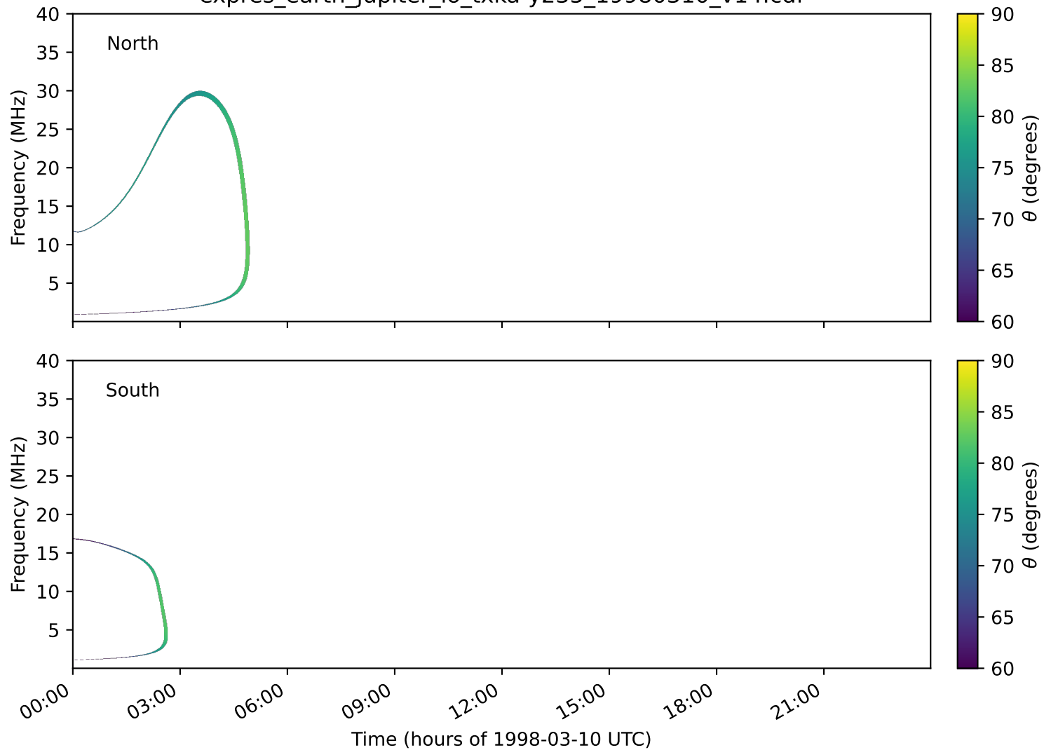
expres_earth_jupiter_io_txka-y235_19980310_v14.cdf
