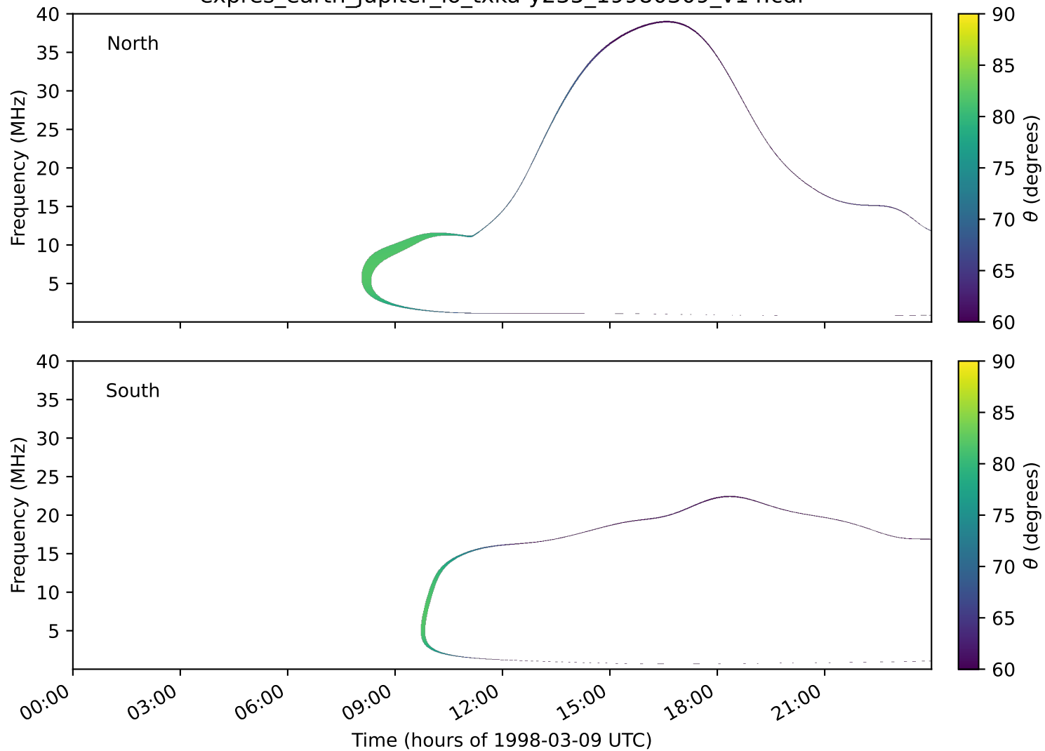
expres_earth_jupiter_io_txka-y235_19980309_v14.cdf
