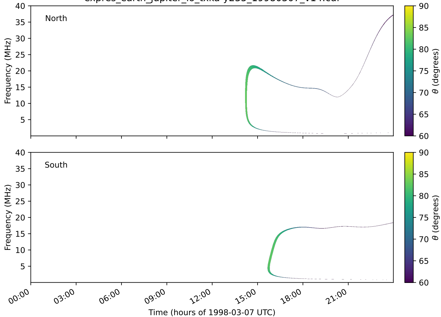
expres_earth_jupiter_io_txka-y235_19980307_v14.cdf
