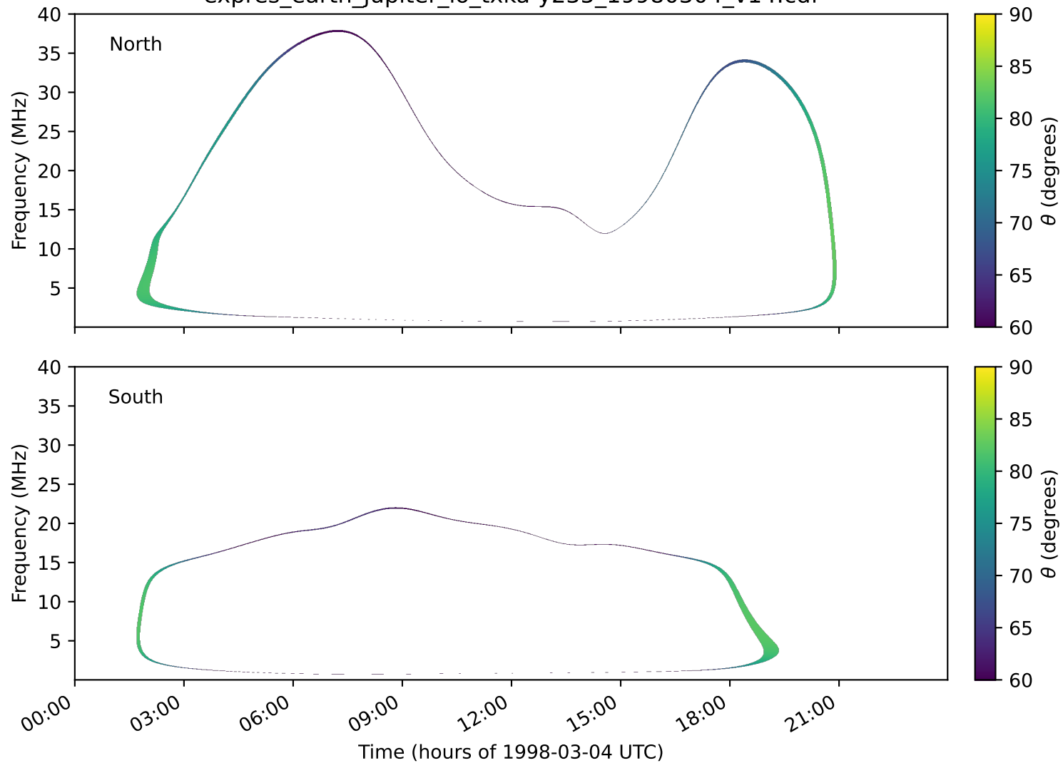
expres_earth_jupiter_io_txka-y235_19980304_v14.cdf
