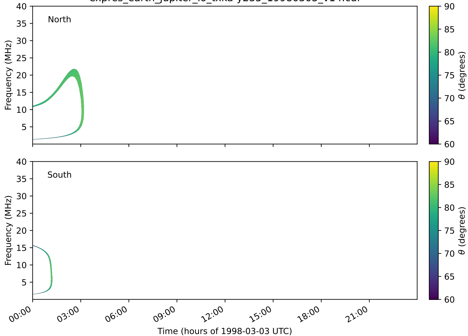
expres_earth_jupiter_io_txka-y235_19980303_v14.cdf
