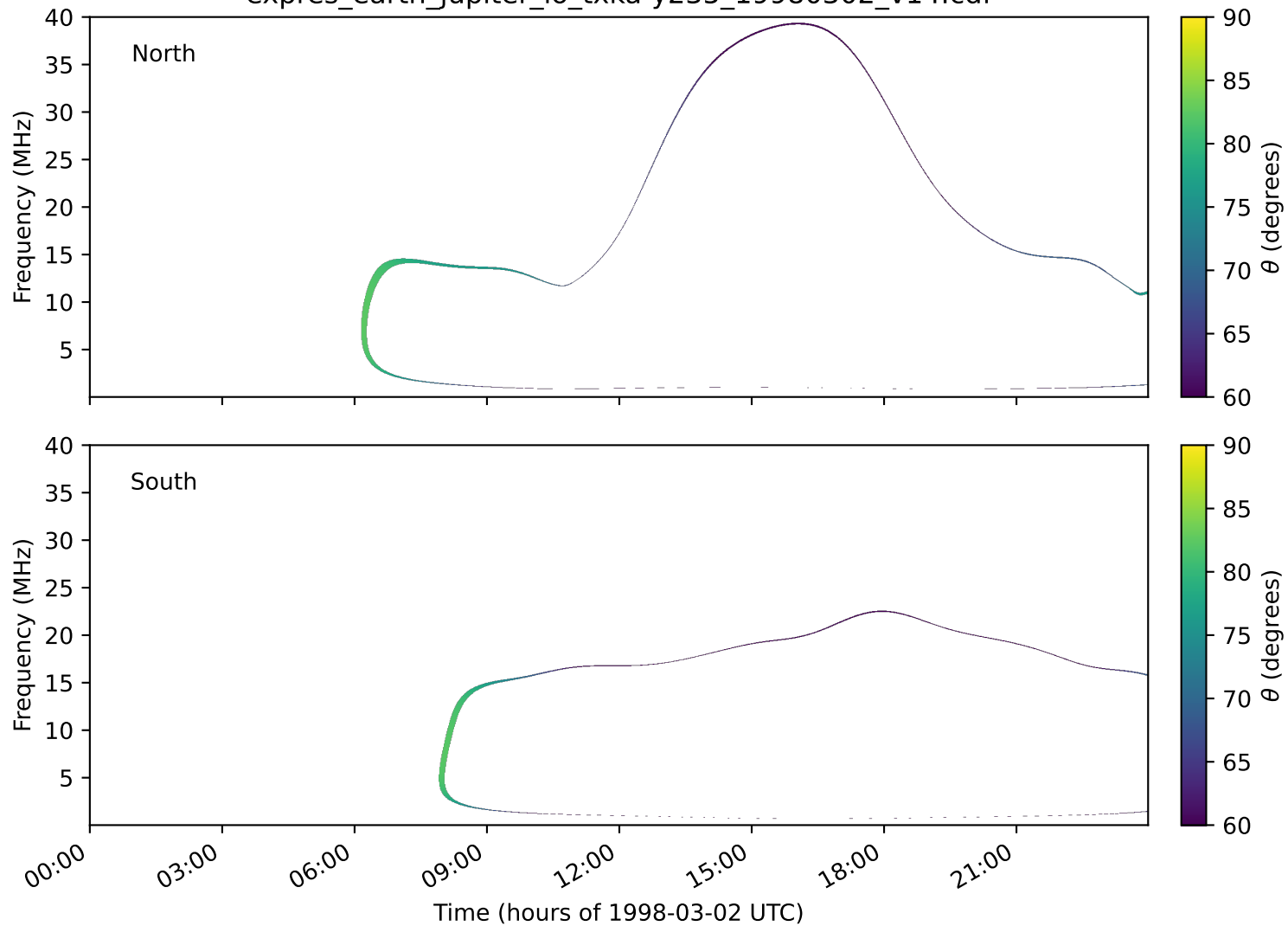
expres_earth_jupiter_io_txka-y235_19980302_v14.cdf
