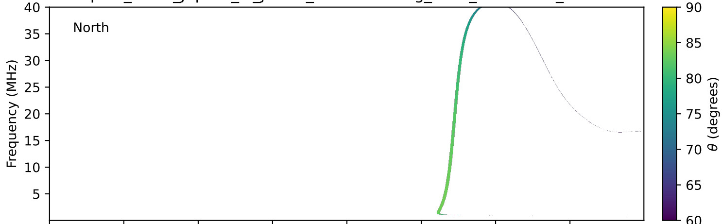
expres_earth_jupiter_io_jrm33_lossc-wid1deg_3kev_19980330_v11.cdf
