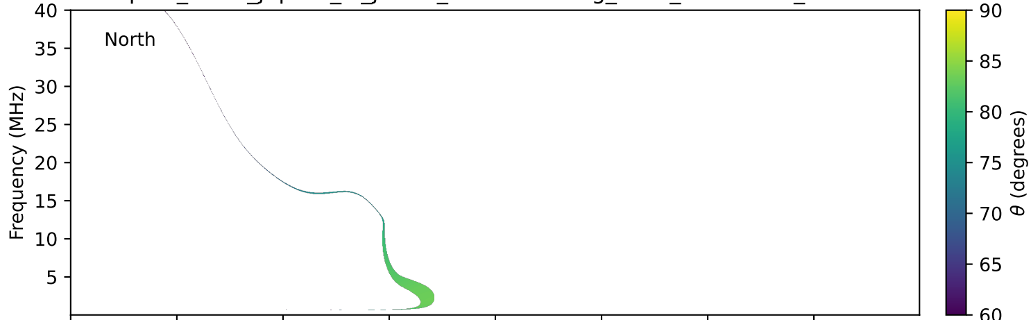
expres_earth_jupiter_io_jrm33_lossc-wid1deg_3kev_19980308_v11.cdf
