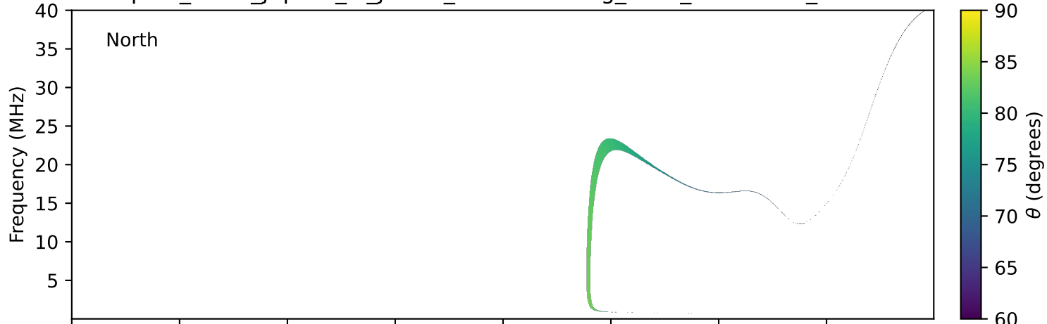
expres_earth_jupiter_io_jrm33_lossc-wid1deg_3kev_19980307_v11.cdf
