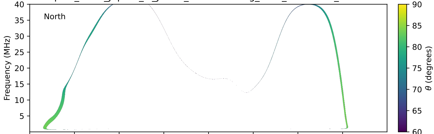
expres_earth_jupiter_io_jrm33_lossc-wid1deg_3kev_19980304_v11.cdf
