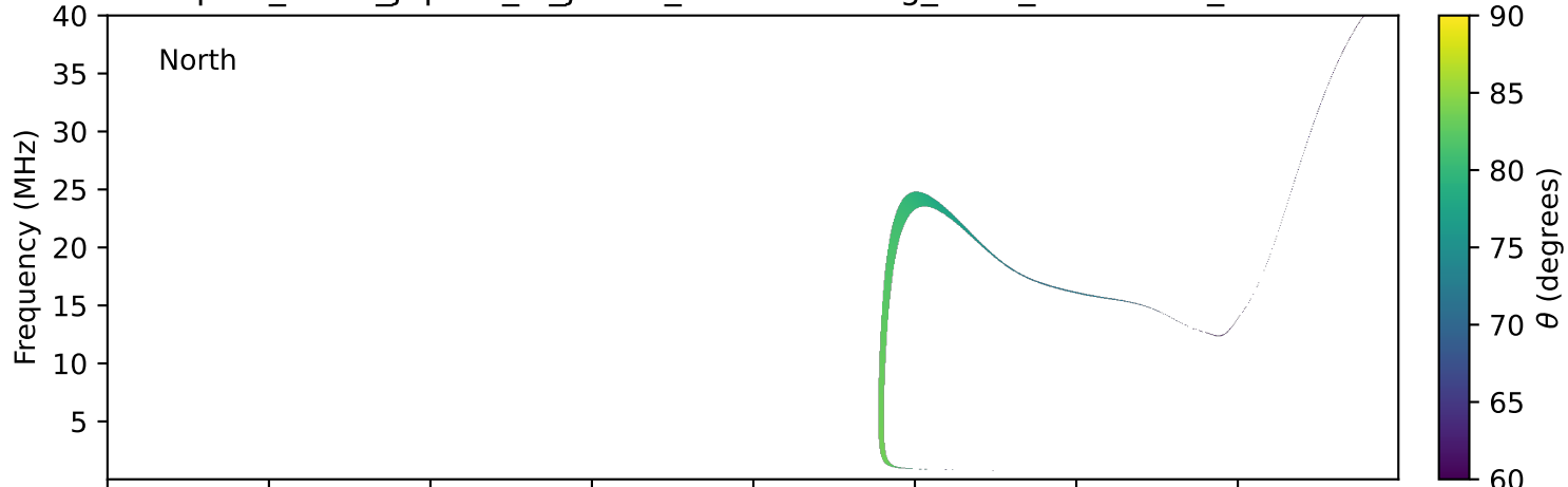
expres_earth_jupiter_io_jrm09_lossc-wid1deg_3kev_19980307_v11.cdf
