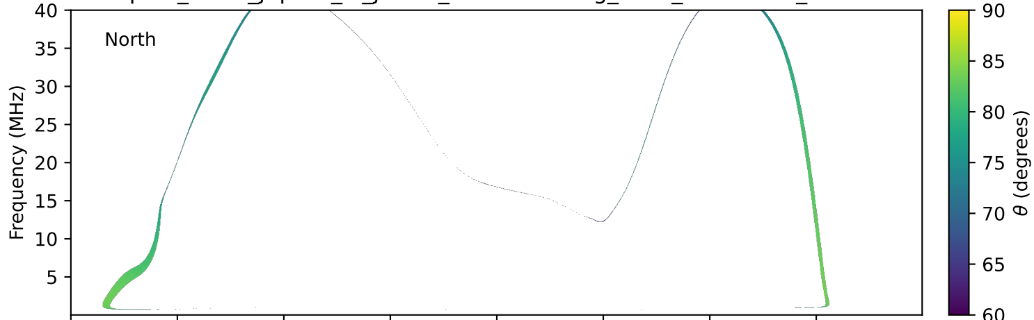
expres_earth_jupiter_io_jrm09_lossc-wid1deg_3kev_19980304_v11.cdf
