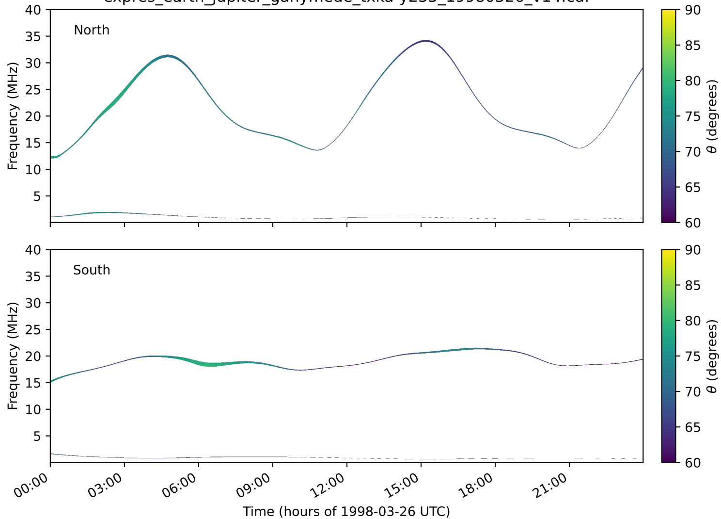
expres_earth_jupiter_ganymede_txka-y235_19980326_v14.cdf
