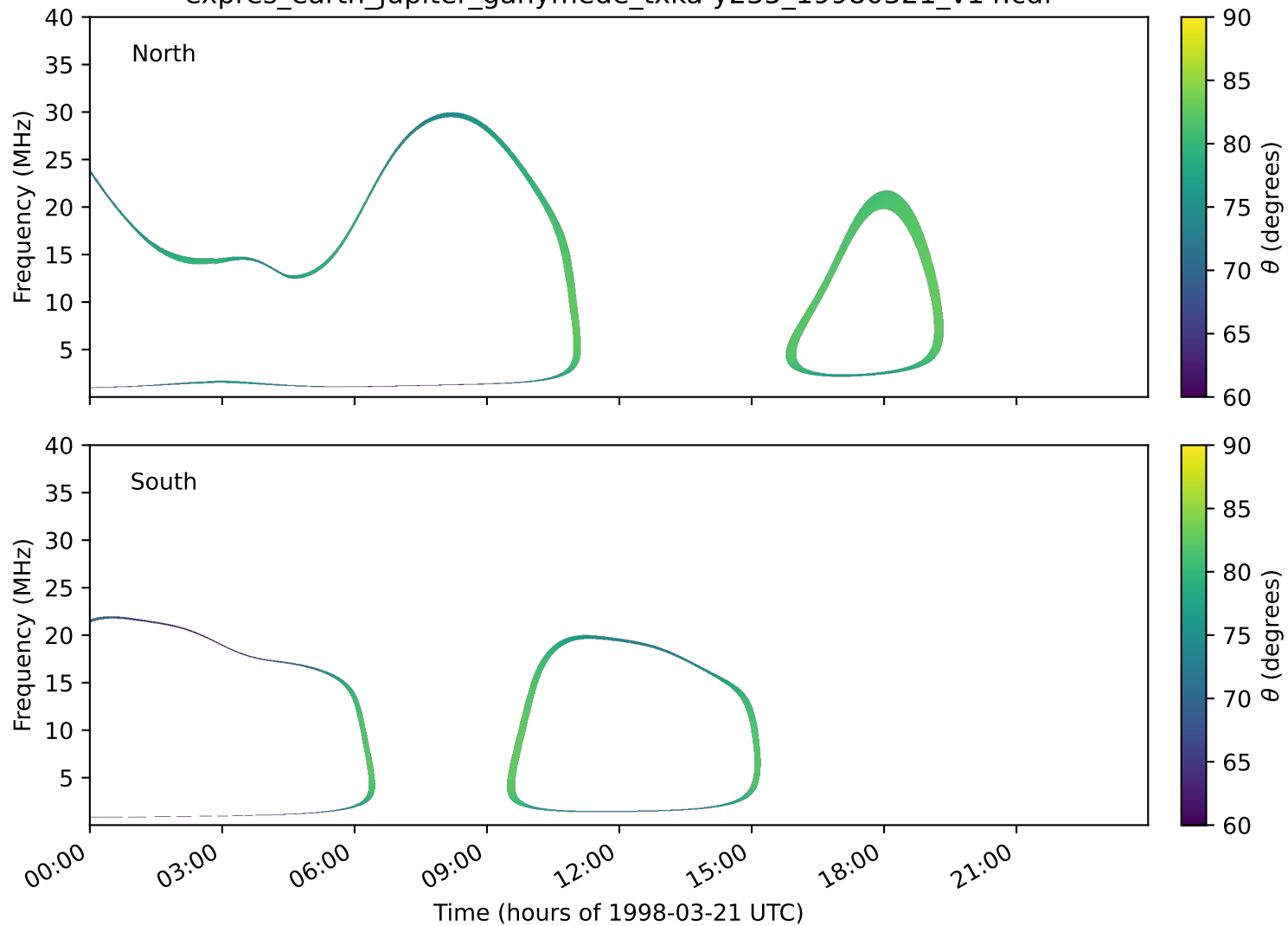
expres_earth_jupiter_ganymede_txka-y235_19980321_v14.cdf
