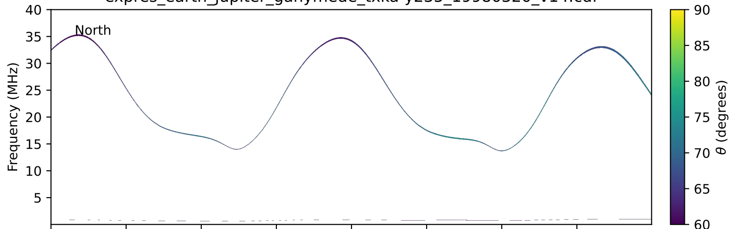
expres_earth_jupiter_ganymede_txka-y235_19980320_v14.cdf
