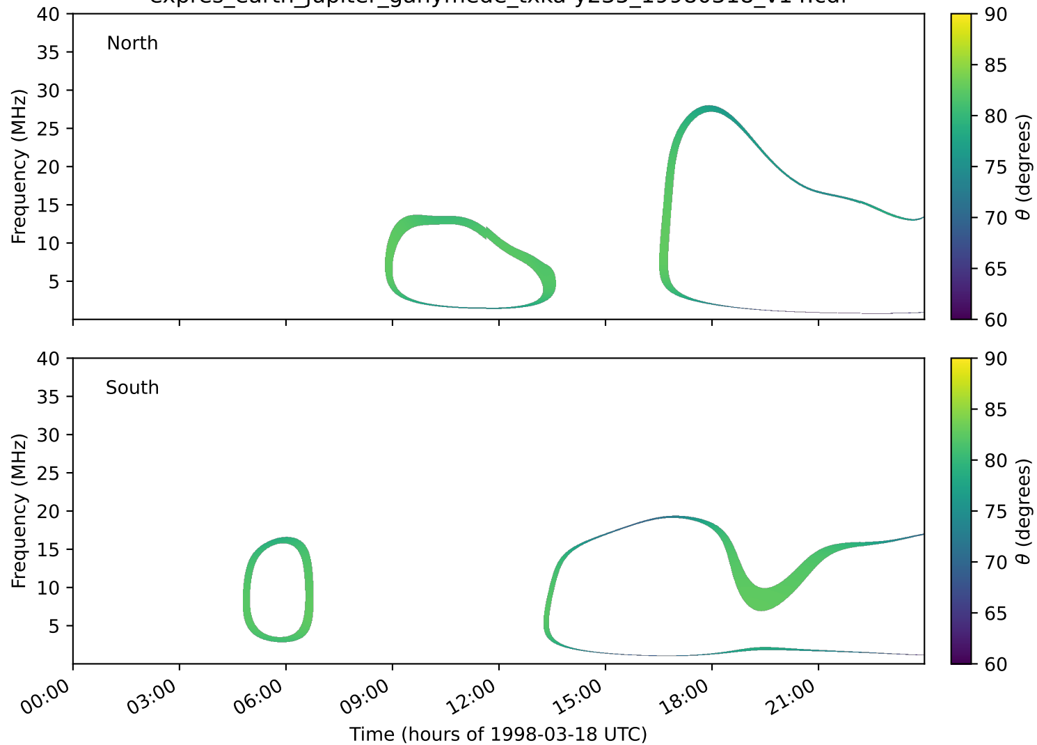
expres_earth_jupiter_ganymede_txka-y235_19980318_v14.cdf
