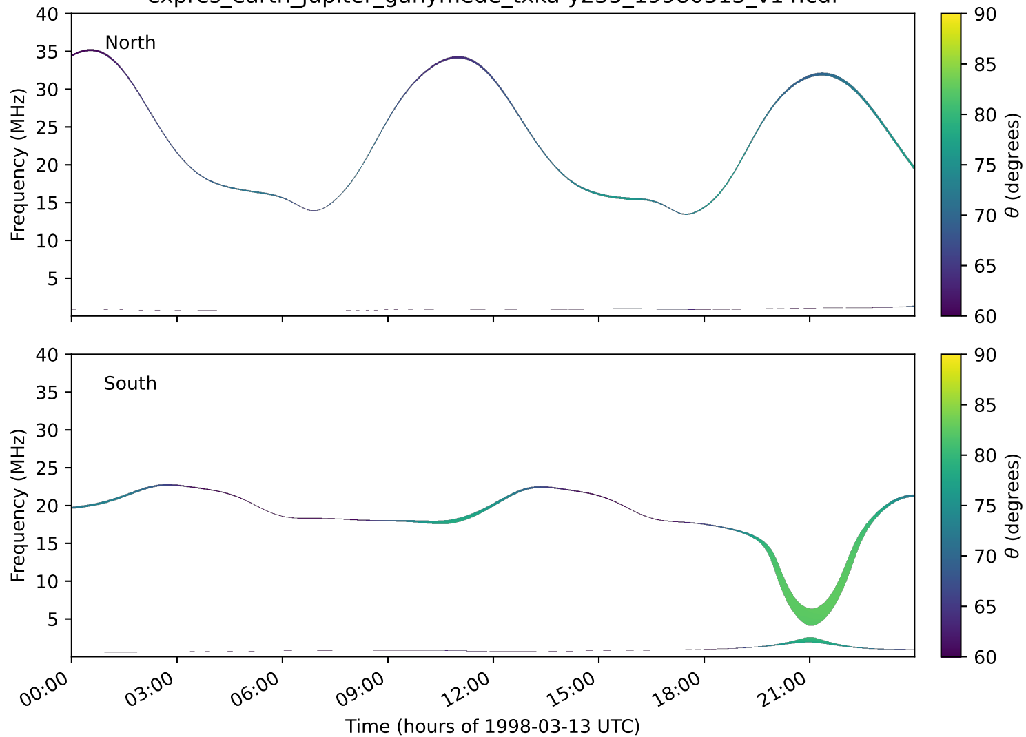
expres_earth_jupiter_ganymede_txka-y235_19980313_v14.cdf
