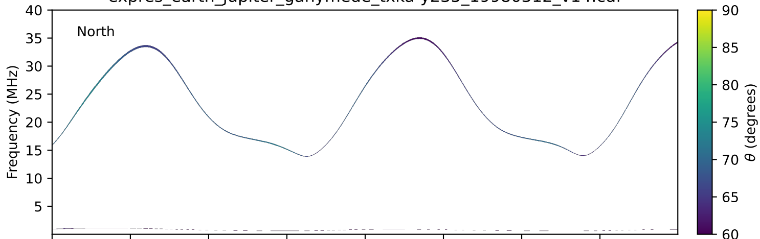
expres_earth_jupiter_ganymede_txka-y235_19980312_v14.cdf
