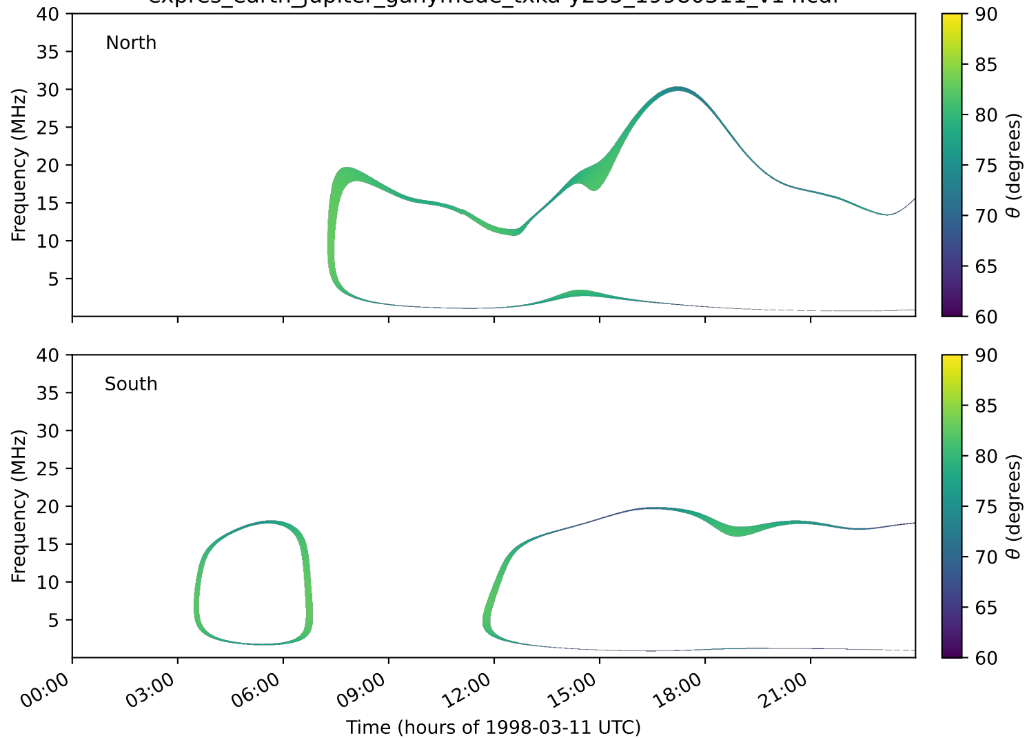
expres_earth_jupiter_ganymede_txka-y235_19980311_v14.cdf
