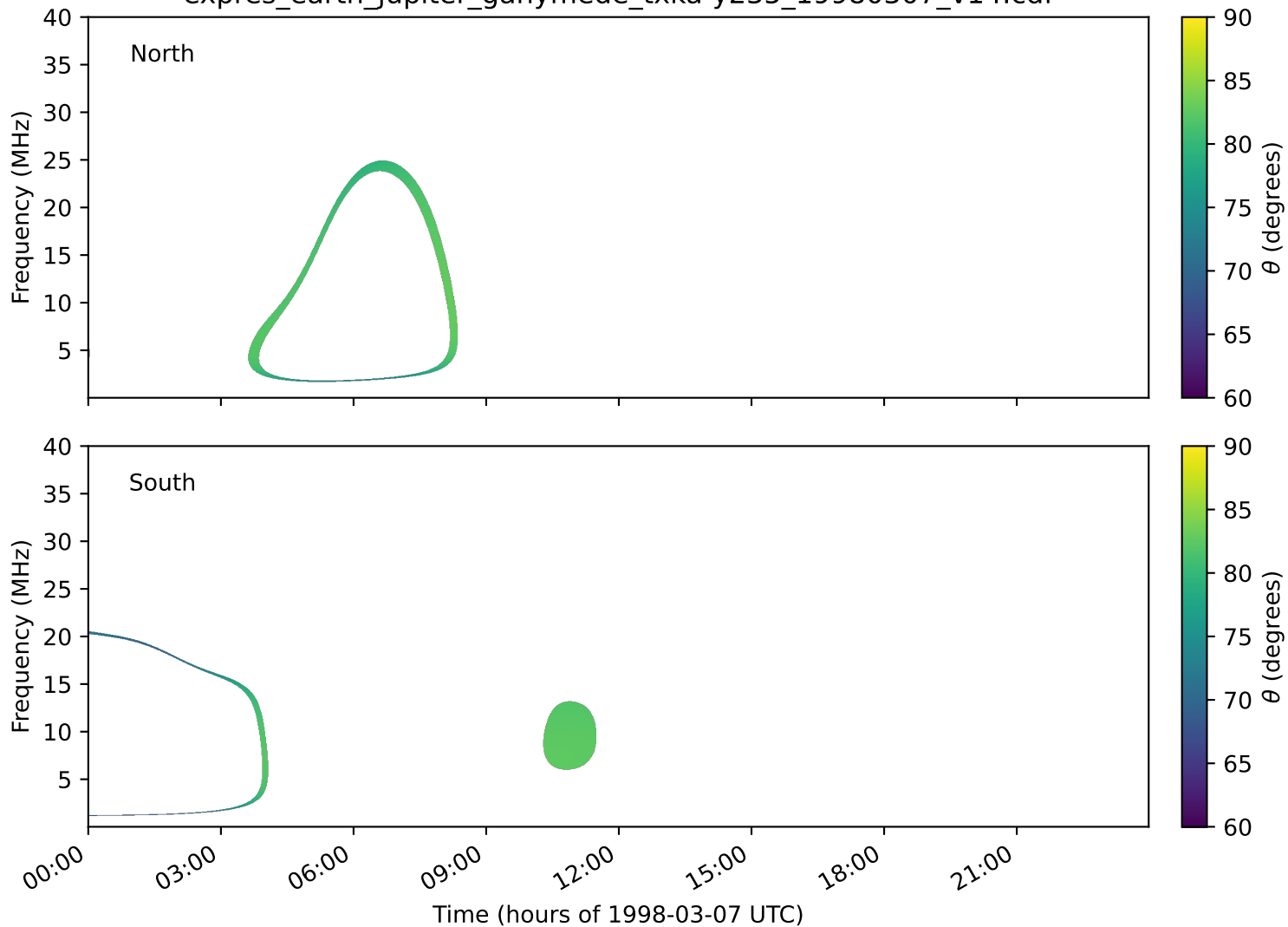
expres_earth_jupiter_ganymede_txka-y235_19980307_v14.cdf
