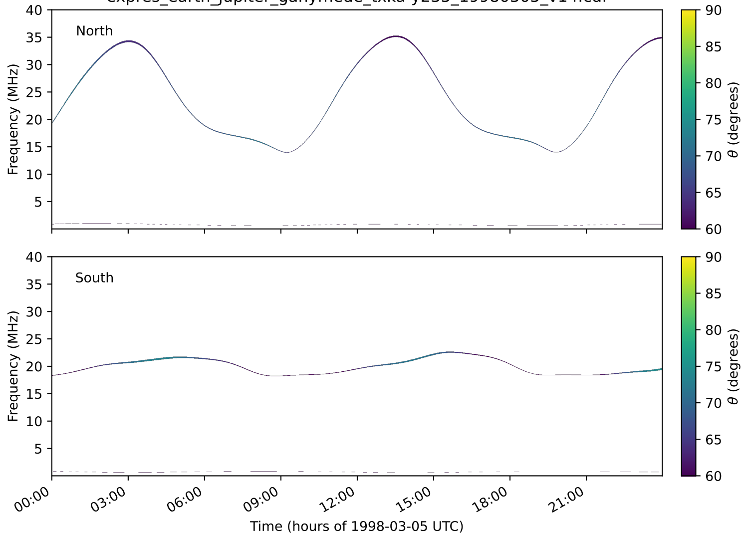
expres_earth_jupiter_ganymede_txka-y235_19980305_v14.cdf
