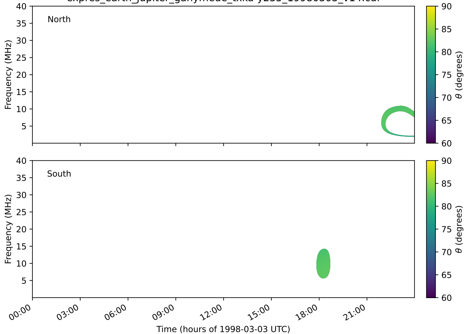
expres_earth_jupiter_ganymede_txka-y235_19980303_v14.cdf
