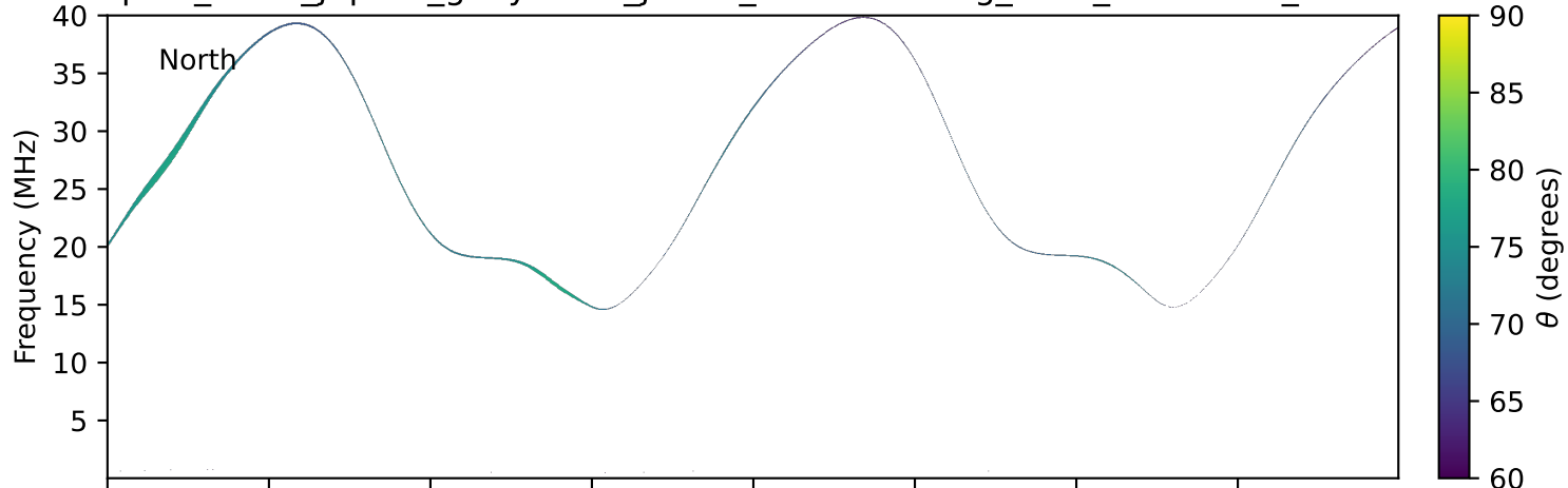
expres_earth_jupiter_ganymede_jrm33_lossc-wid1deg_3kev_19980312_v11.cdf
