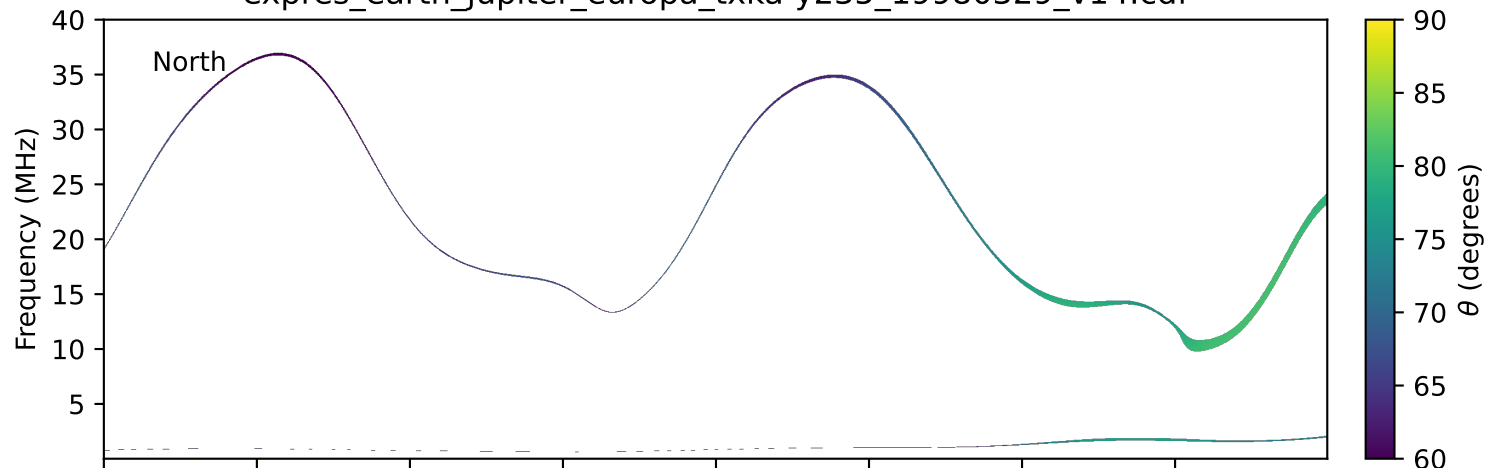
expres_earth_jupiter_europa_txka-y235_19980329_v14.cdf
