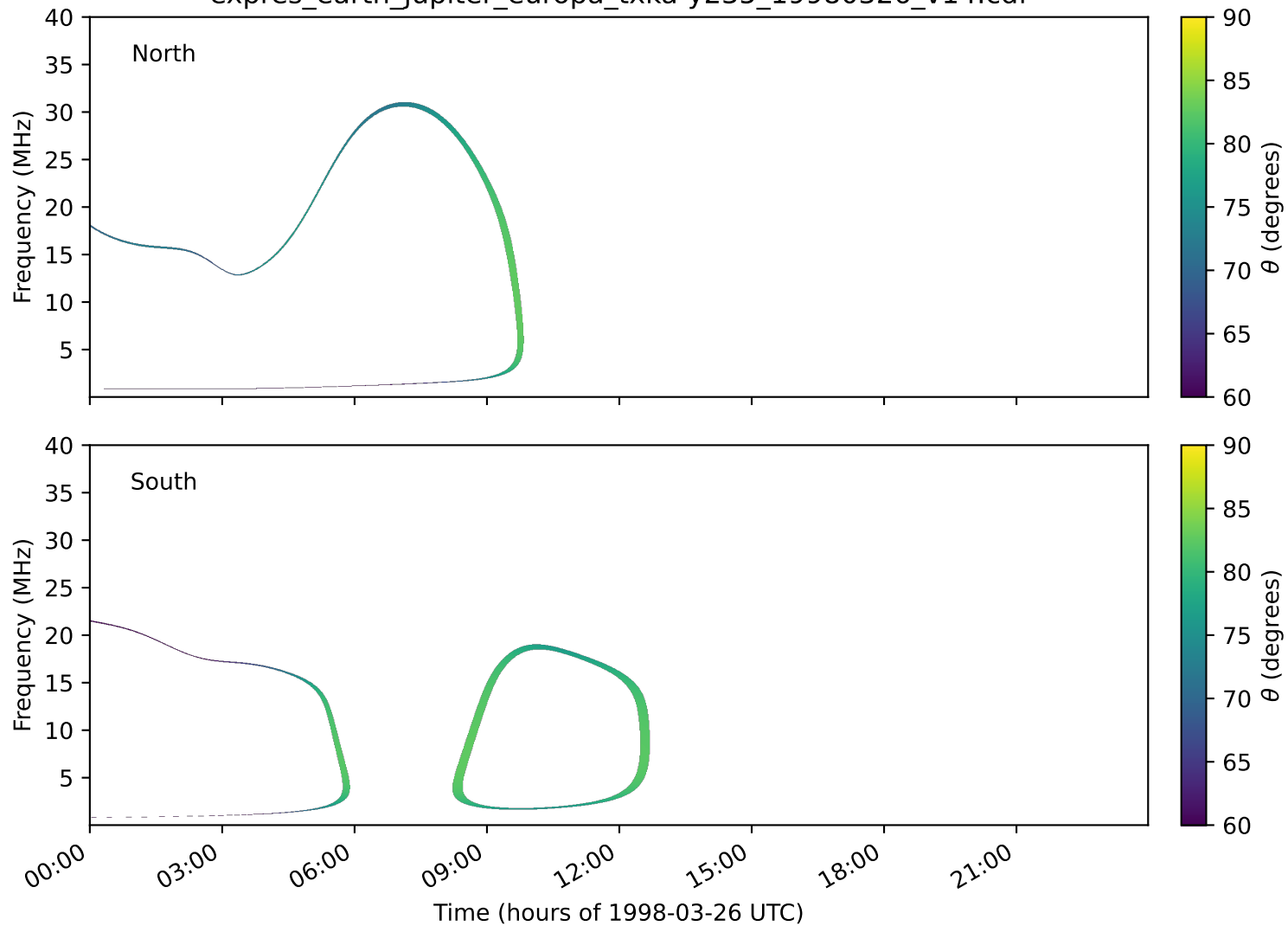
expres_earth_jupiter_europa_txka-y235_19980326_v14.cdf
