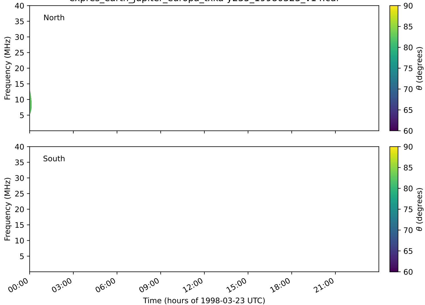
expres_earth_jupiter_europa_txka-y235_19980323_v14.cdf
