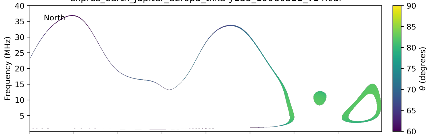
expres_earth_jupiter_europa_txka-y235_19980322_v14.cdf
