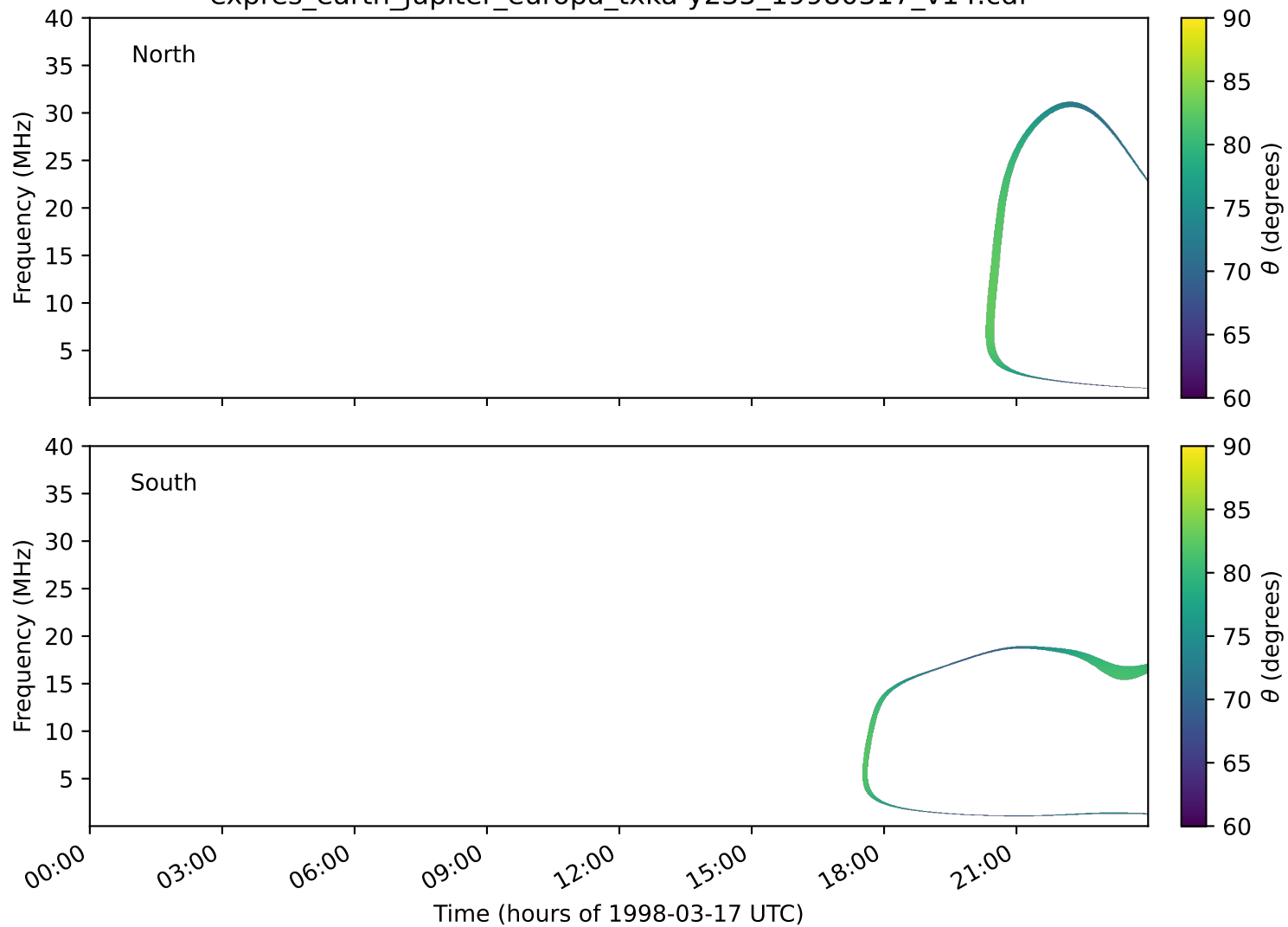
expres_earth_jupiter_europa_txka-y235_19980317_v14.cdf
