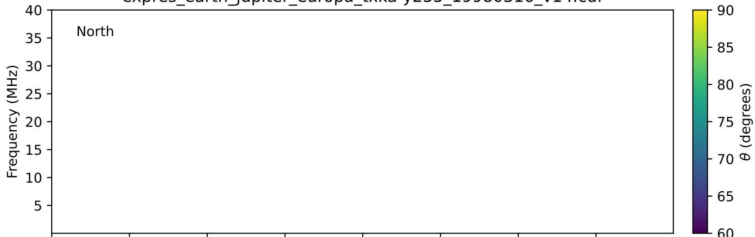
expres_earth_jupiter_europa_txka-y235_19980316_v14.cdf
