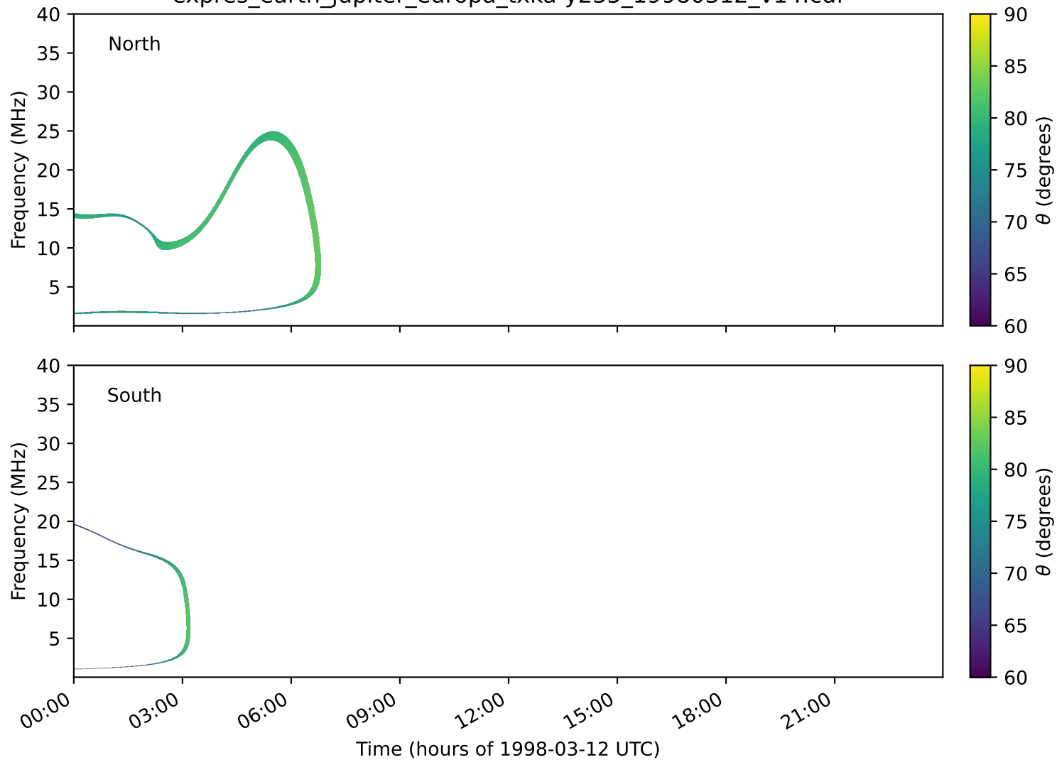
expres_earth_jupiter_europa_txka-y235_19980312_v14.cdf
