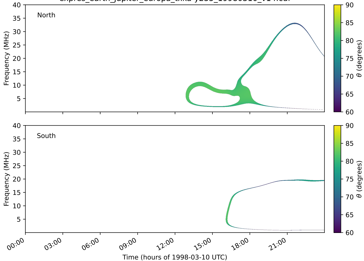
expres_earth_jupiter_europa_txka-y235_19980310_v14.cdf
