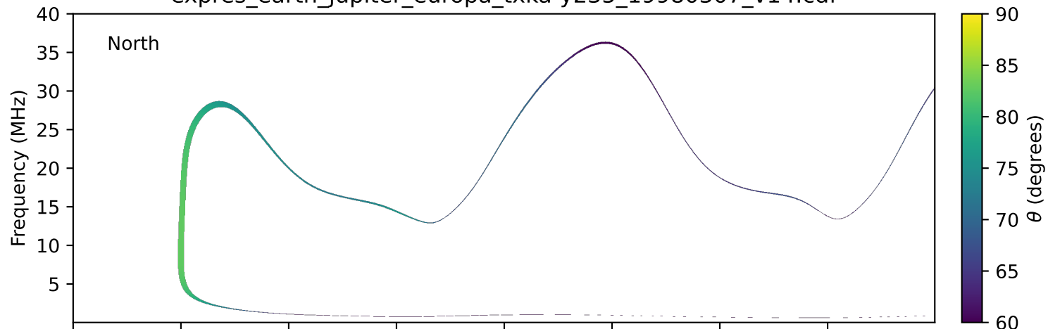
expres_earth_jupiter_europa_txka-y235_19980307_v14.cdf
