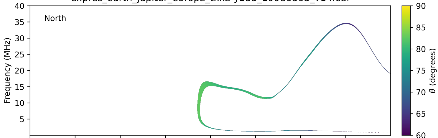
expres_earth_jupiter_europa_txka-y235_19980303_v14.cdf
