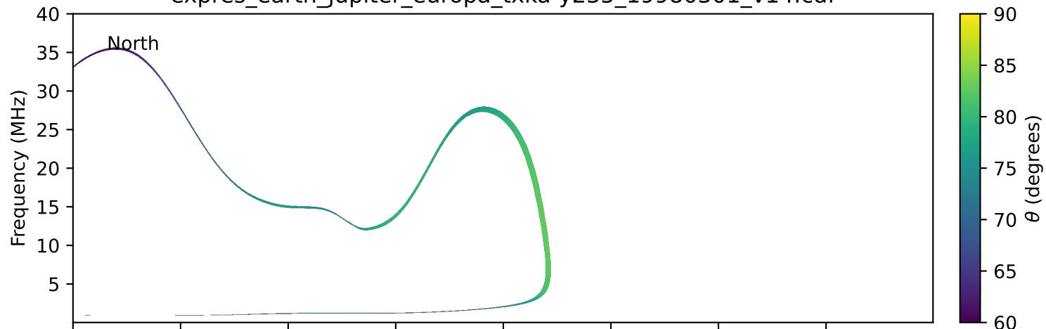
expres_earth_jupiter_europa_txka-y235_19980301_v14.cdf
