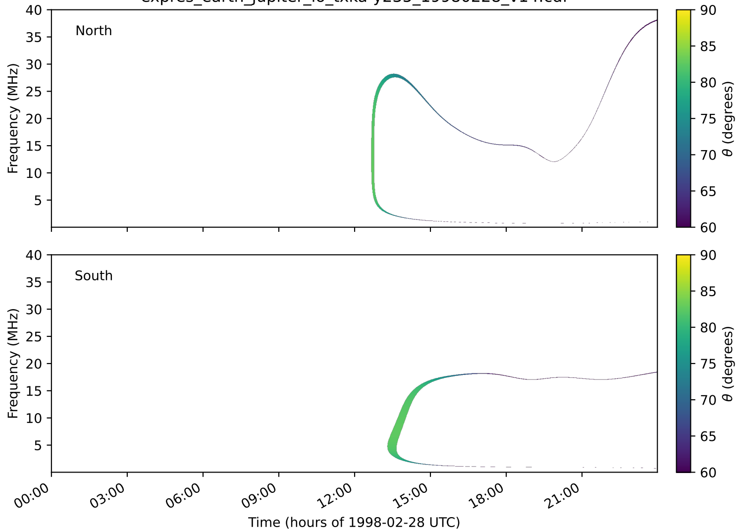
expres_earth_jupiter_io_txka-y235_19980228_v14.cdf
