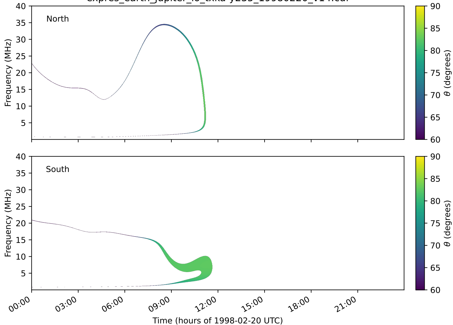
expres_earth_jupiter_io_txka-y235_19980220_v14.cdf
