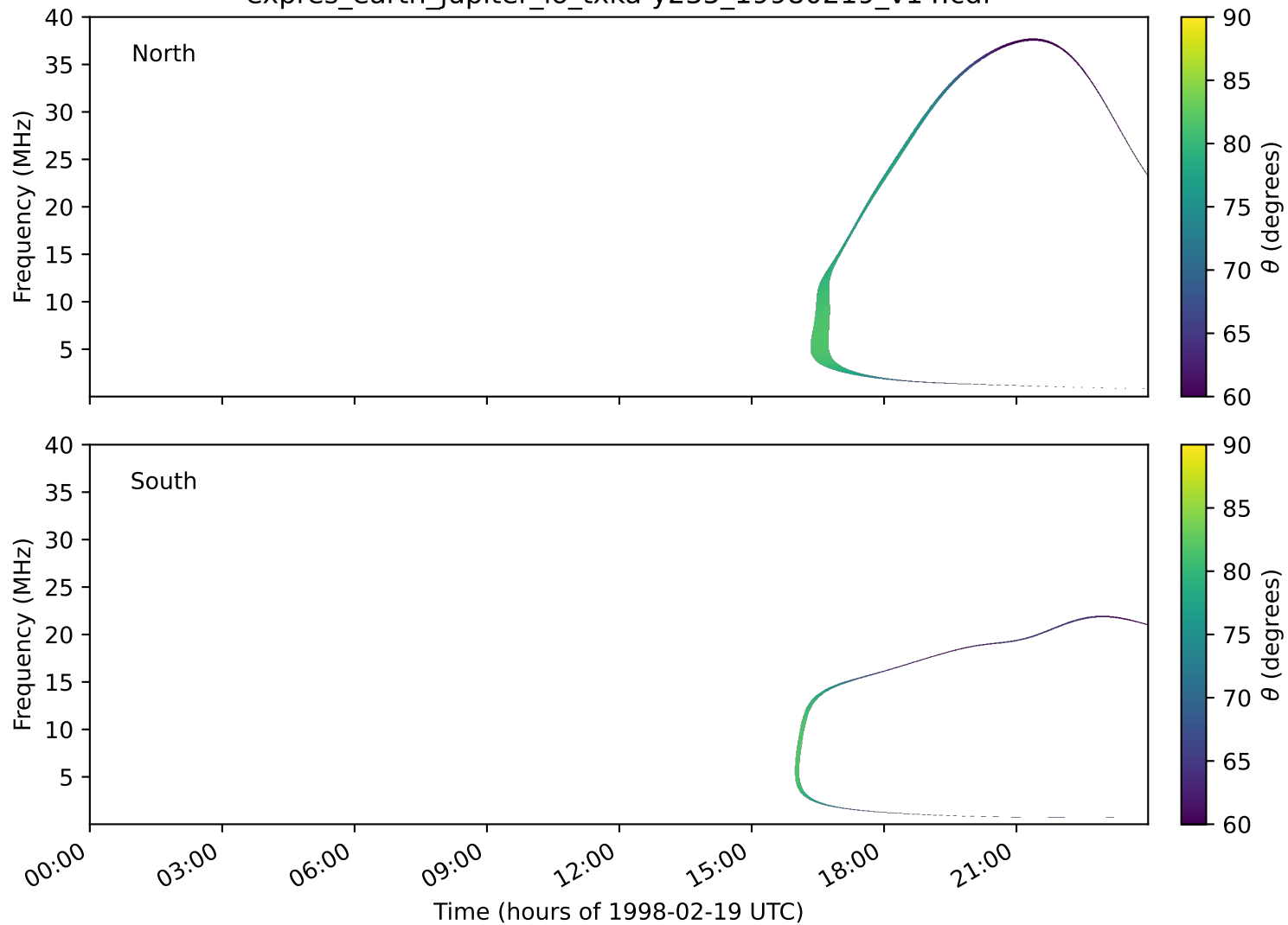
expres_earth_jupiter_io_txka-y235_19980219_v14.cdf
